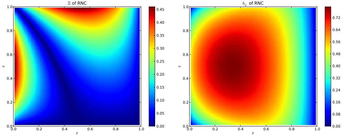
Figure 4: Invariants of the RnC process over the space of p, q values
