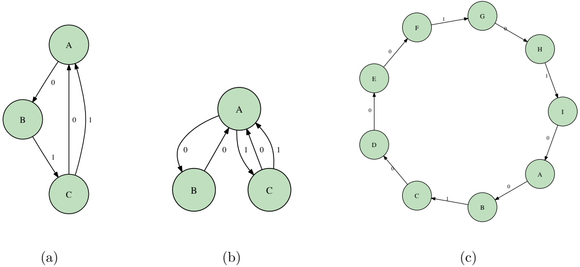
Figure 8: Examples of discrete finite automata with binary alphabets, showing similarities to graph presentations of \epsilon -machines without transition probabilities
